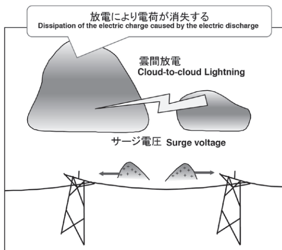
図2 (a) 静電誘導サージ Fig. 2(a) Electrostatic induction surge
