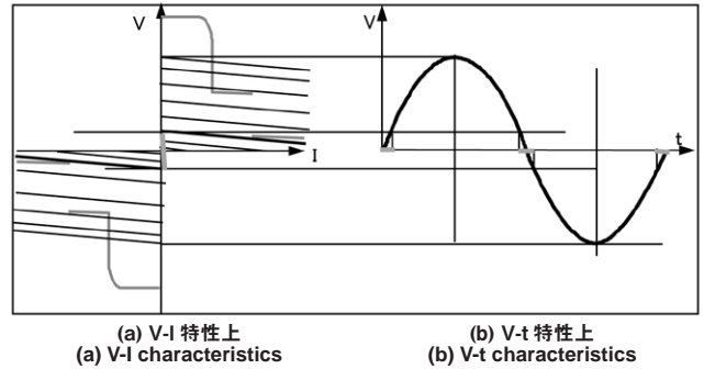
図 15 抵抗が小さい時 (続流不可能領域が短い) Fig.15 At Low Resistance (Short Range of No Follow-on-current)
