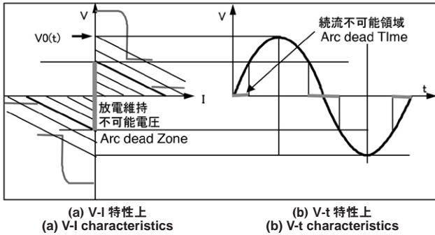
図 14 抵抗が大きい時 (続流不可能領域が長い) Fig.14 At High Resistance (Long Range of No Follow-on-current)
