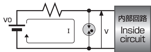
図13 電源の出力特性 Fig.13 Output characteristic of the power supply
