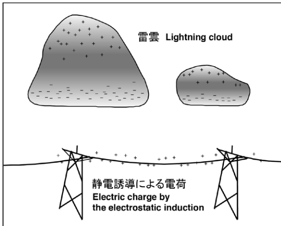
図2 (a) 静電誘導サージ Fig. 2(a) Electrostatic induction surge
